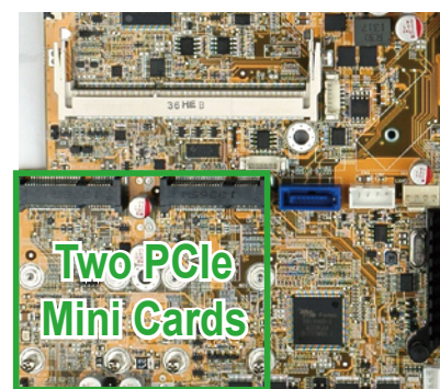
Capture Card Module
