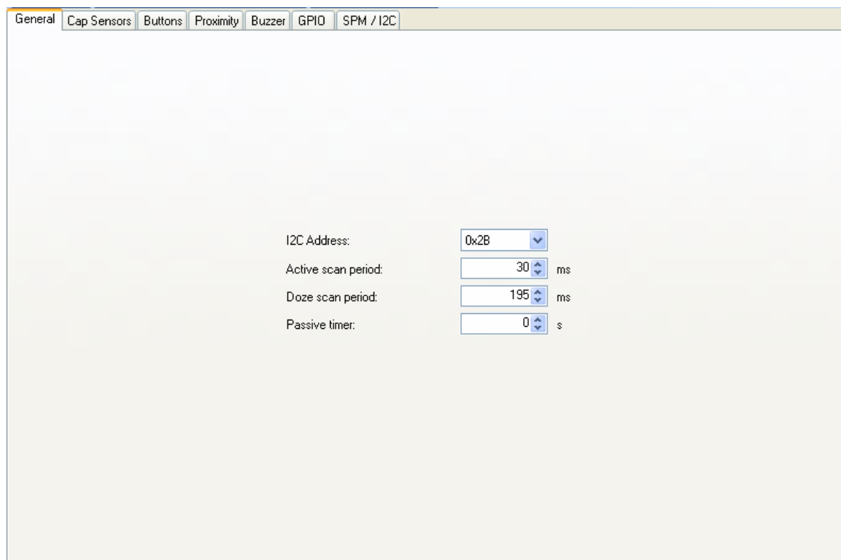
Figure 32: General Tab
