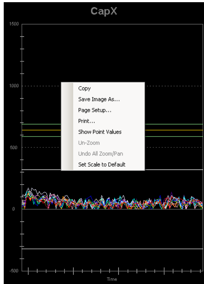
Figure 38: Graph Window
