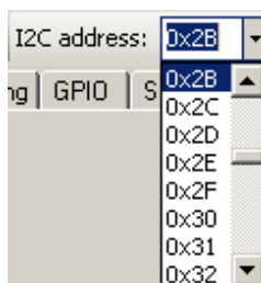
Figure 25: I2C Address
