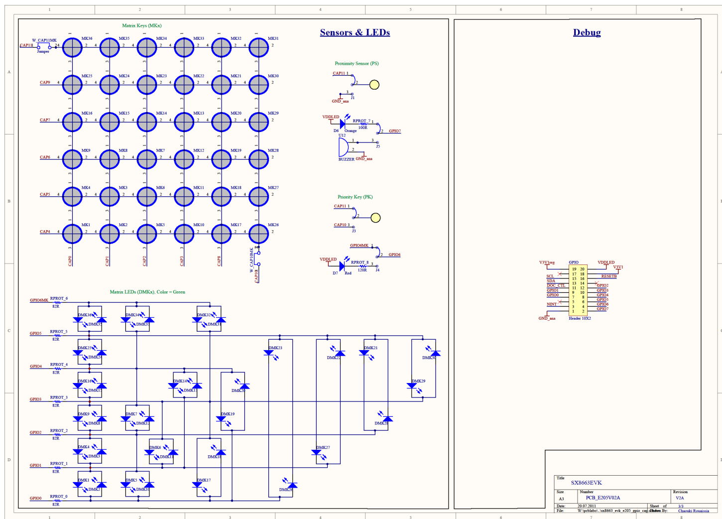
Figure 47: SX8663EVK Schematics (2/2)
