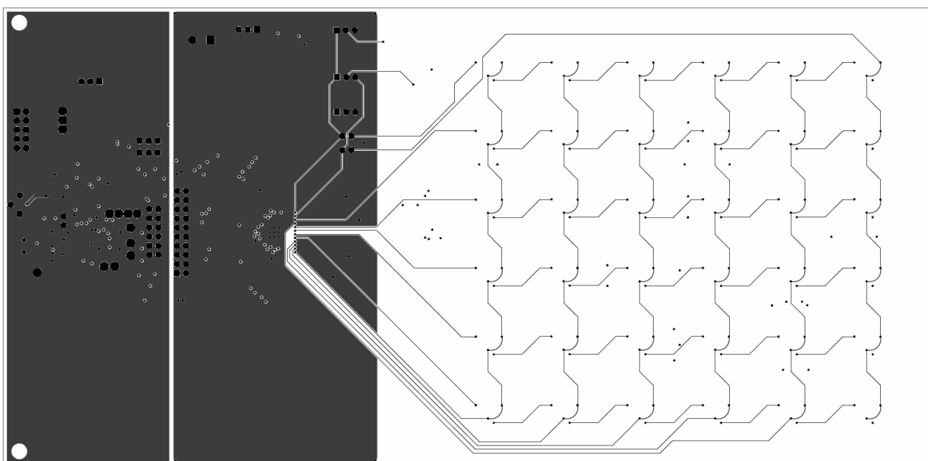
Figure 49: SX8663EVK Mid Layer 1
