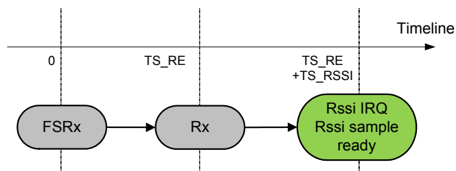
Figure 15. Time to Rssi Sample
