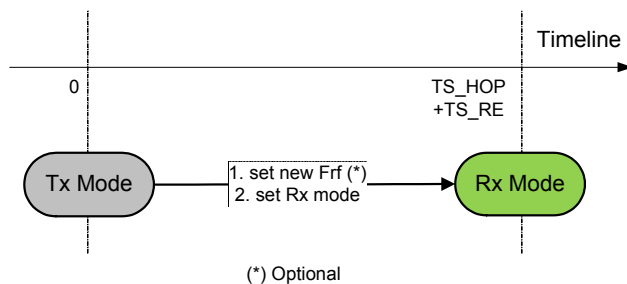
Figure 16. Tx to Rx Turnaround
