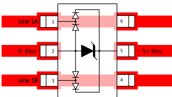
Figure 4 - Dual Voltage Layout Diagram
