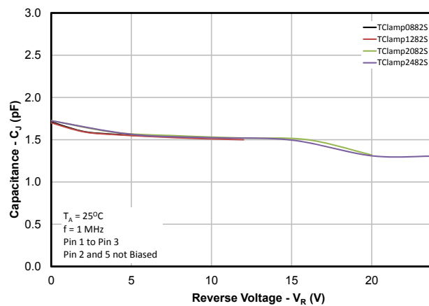
Capacitance vs. Reverse Voltage (Pin 1 to 3)
