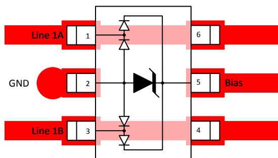
Figure 3 - Single Ended Layout Diagram
