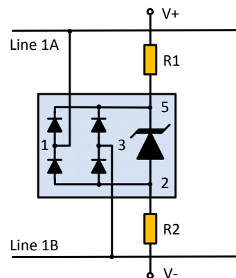
Figure 5 - External Bias Resistors
