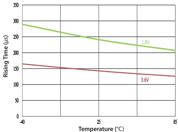
Rising Time vs. Temperature
