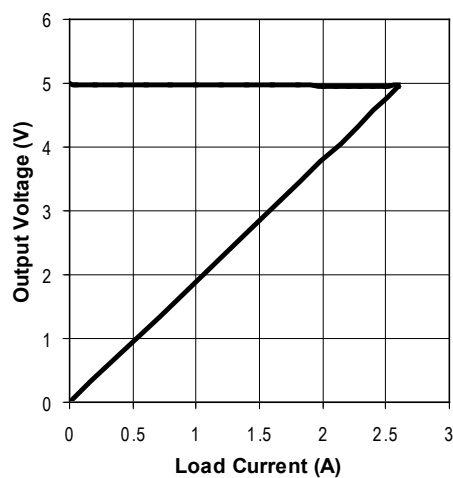
Load Characteristic
