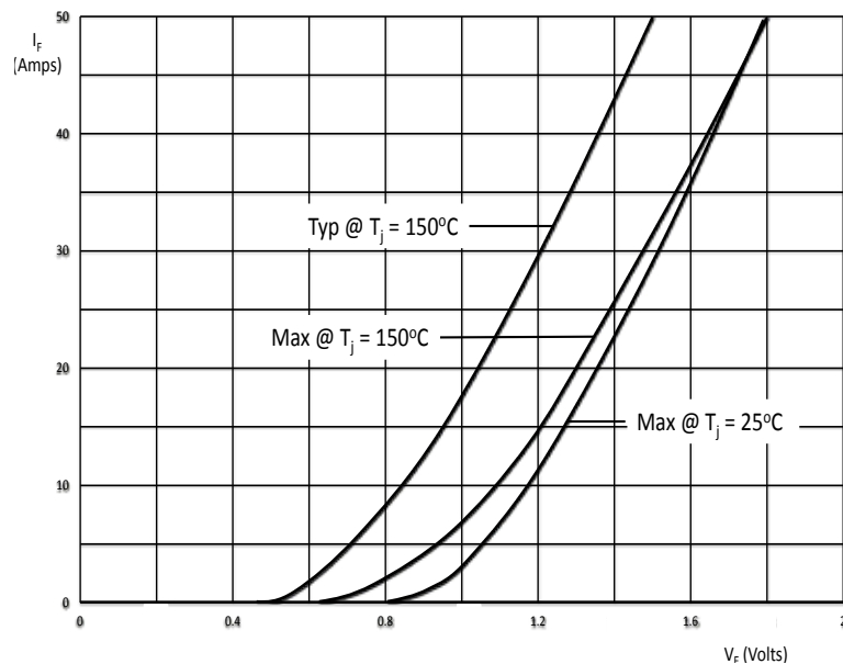
Figure 2. Forward voltage drop per leg as a function of forward current for SET111403 and SET111412
