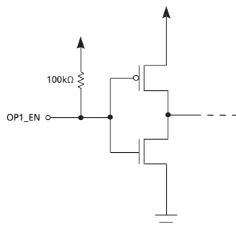
Figure 3-4: OP1_EN Circuit
