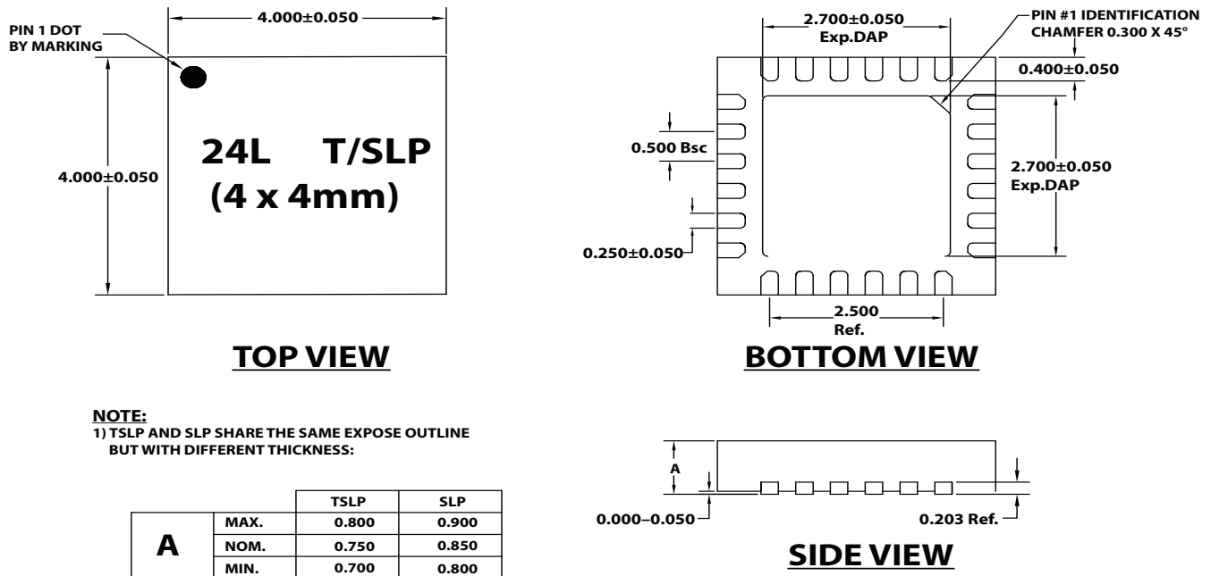
Figure 6-1: Package Dimensions
