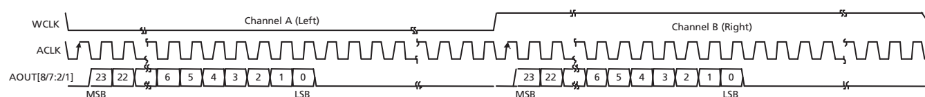
Figure 4-37: I 2 S Audio Output Format
