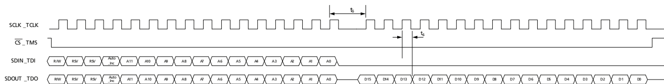
Figure 4-52: Read Mode
