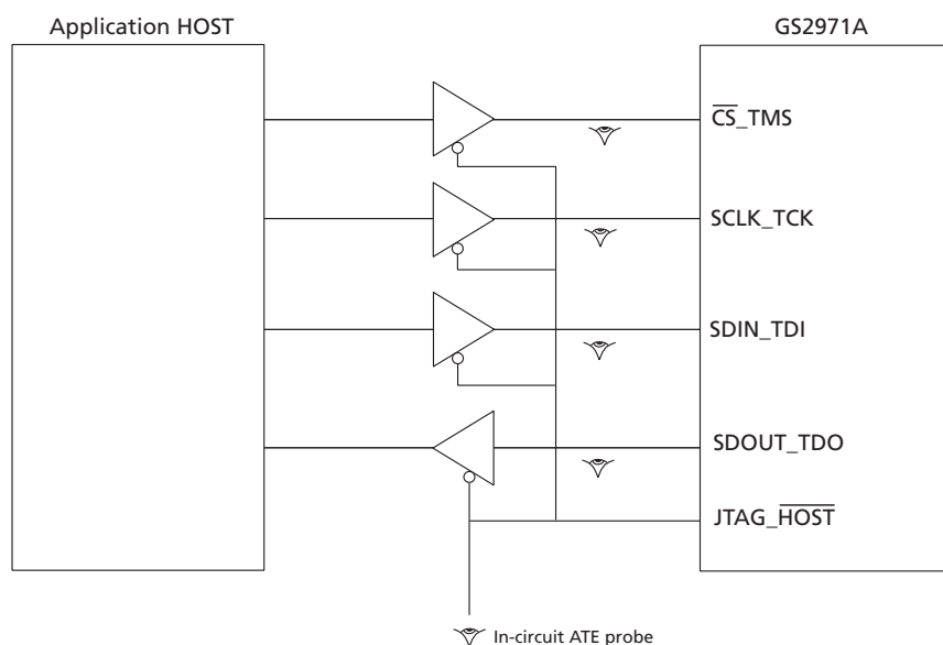
Figure 4-54: In-Circuit JTAG
