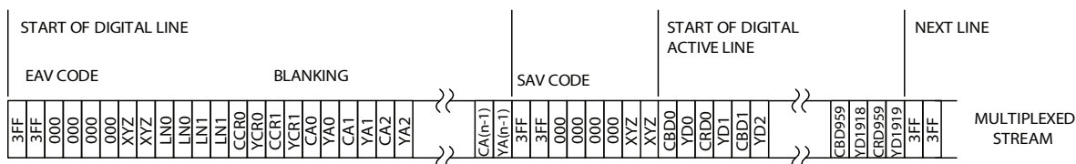
Figure 4-5: Multiplexed Luma and Chroma Over One Video Line - 1080i
