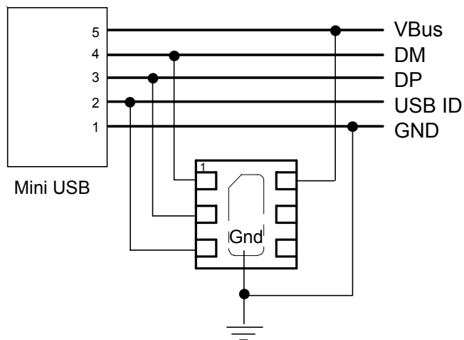
Figure 2 - USB Protection
