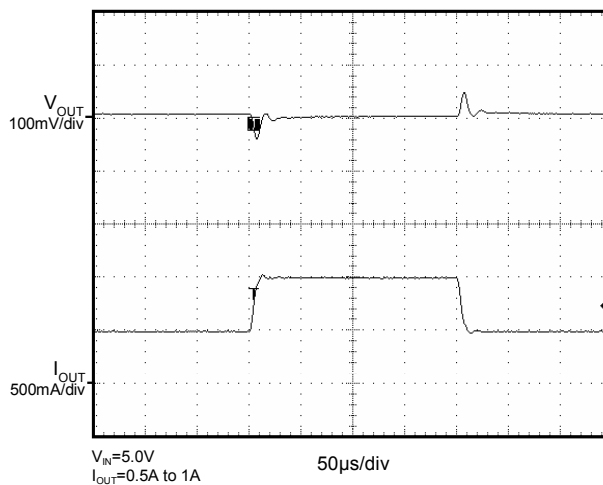
Transient Response ( V_{OUT}=1.5V ; 0.5A to 1.0A)
