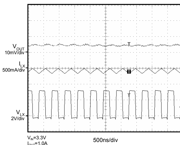
Output Voltage Ripple ( V_{OUT}=1.5V )
