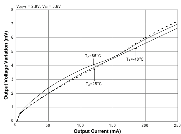
Load Regulation — LDOB
