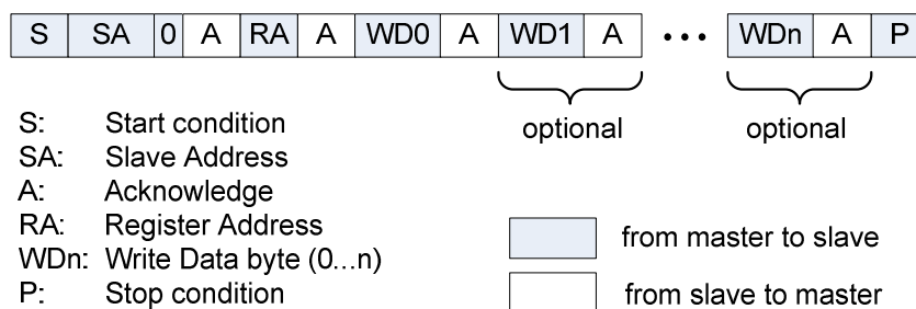
Figure 22: I2C Write
