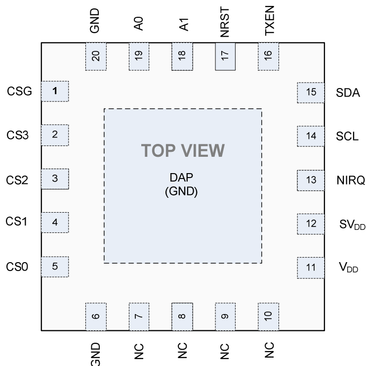
Figure 1: Pin Diagram
