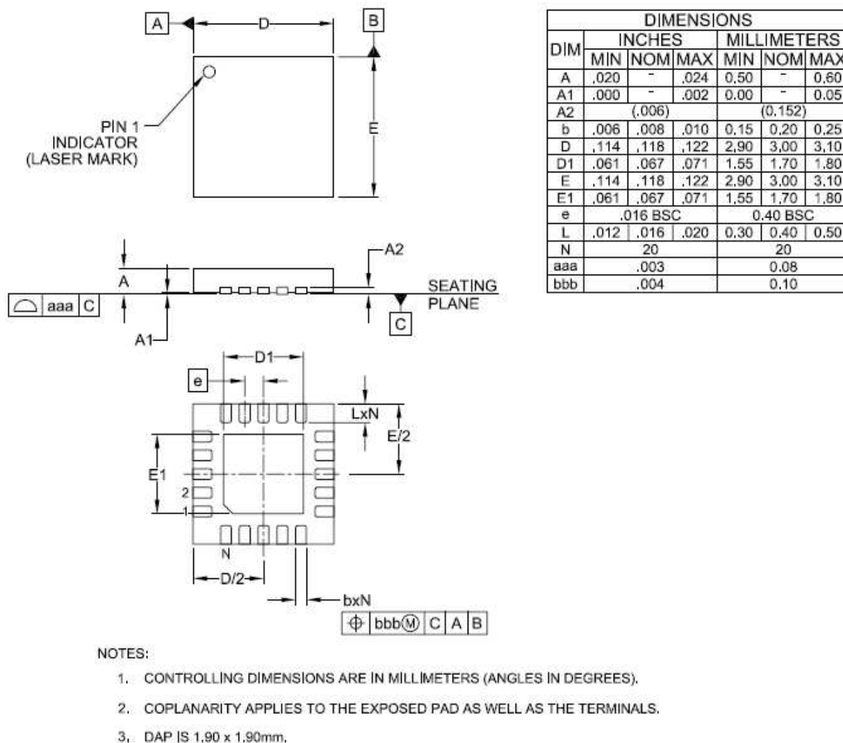
Figure 31: Outline Drawing
