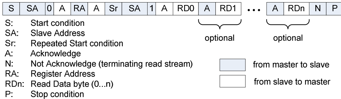
Figure 23: I2C Read
