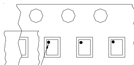
Pin 1 Location
