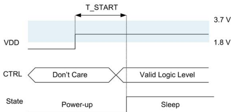
Figure 6. Power-up Timing
