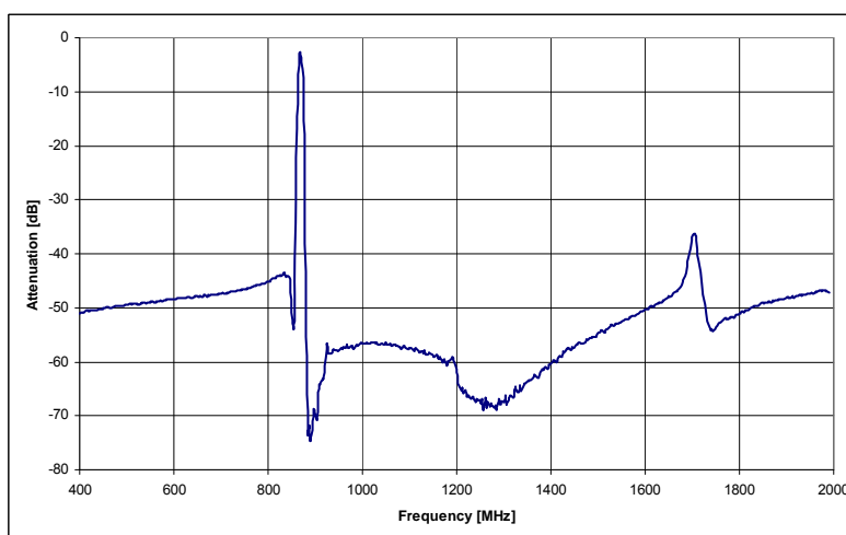
Figure 60: 869 MHz SAW Filter Plot
