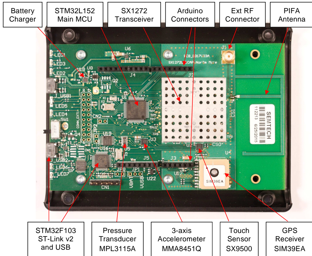
Figure 3 SX1272LM1CEP Details
