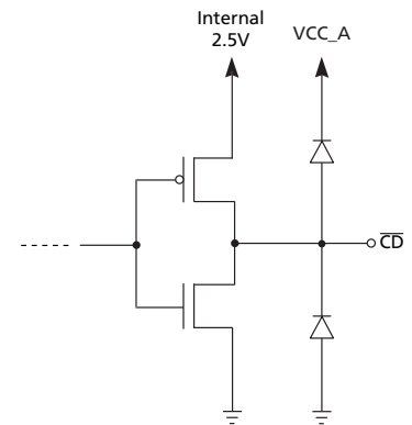
Figure 3-6: \overline{CD} Circuit
