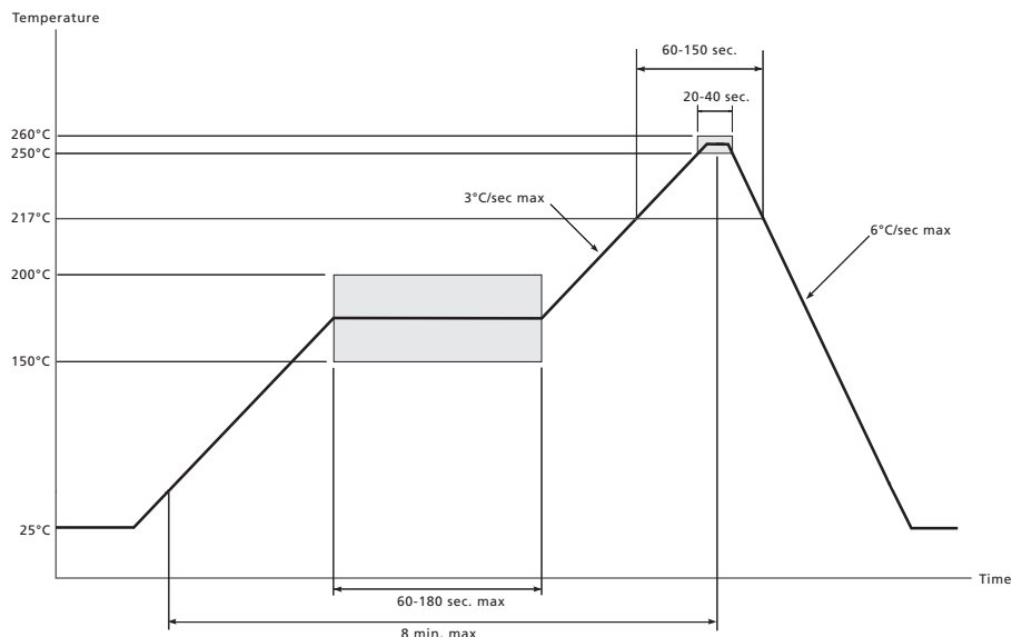
Figure 6-1: Maximum Pb-free Solder Reflow Profile
