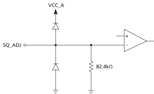
Figure 3-2: SQ_ADJ Equivalent Circuit
