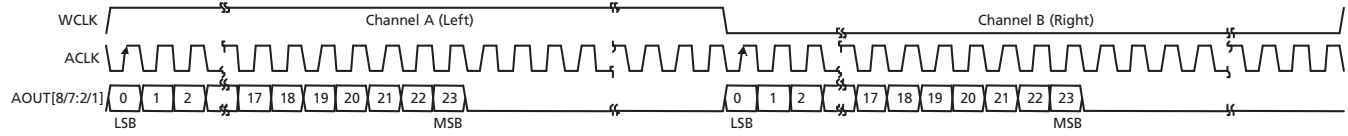
Figure 4-37: Serial Audio, Left Justified, LSB First
