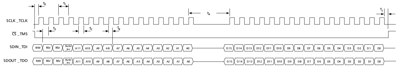
Figure 4-48: Write Mode
