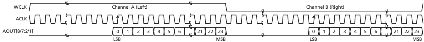
Figure 4-39: Serial Audio, Right Justified, LSB First
