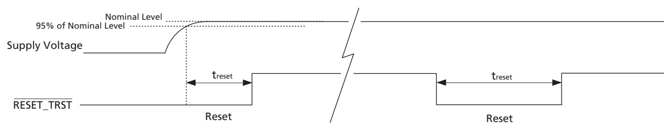
Figure 4-53: Reset Pulse
