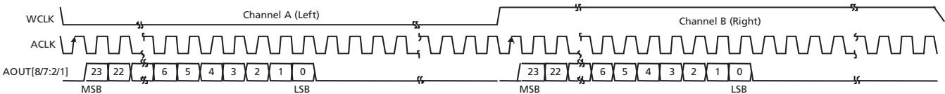
Figure 4-34: I 2 S Audio Output Format
