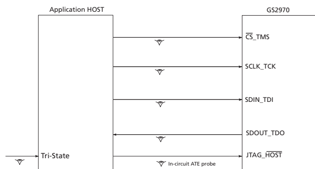
Figure 4-52: System JTAG
