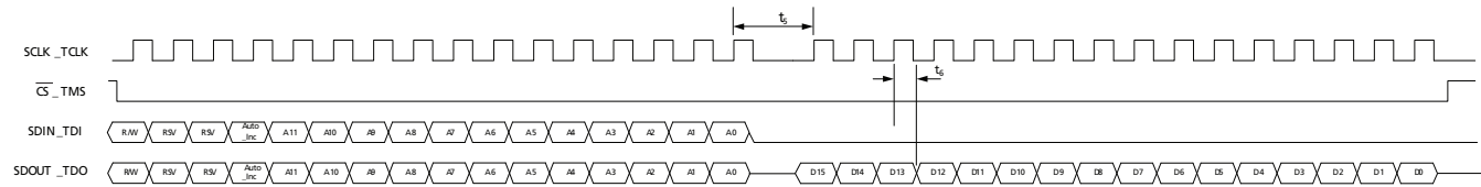
Figure 4-49: Read Mode
