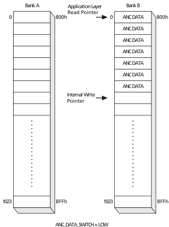
Figure 4-31: Ancillary Data Extraction - Step C
