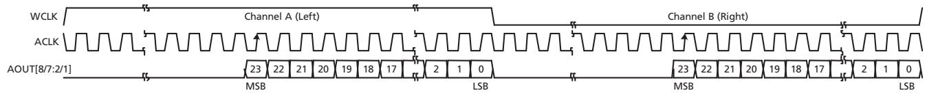
Figure 4-38: Serial Audio, Right Justified, MSB First
