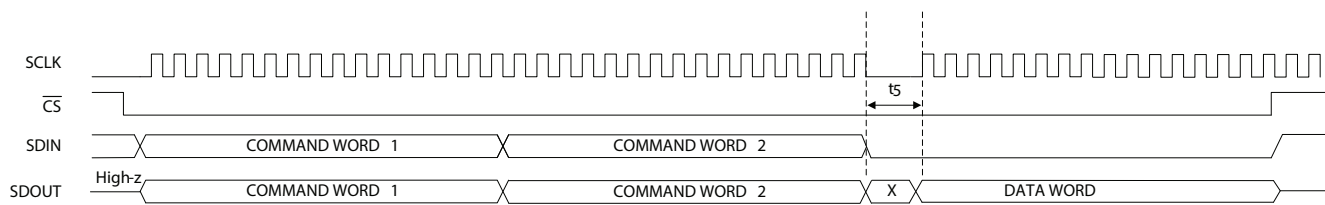
Figure 3-23: GSPI Read Timing—Single Read Access with Bus-Through Operation
