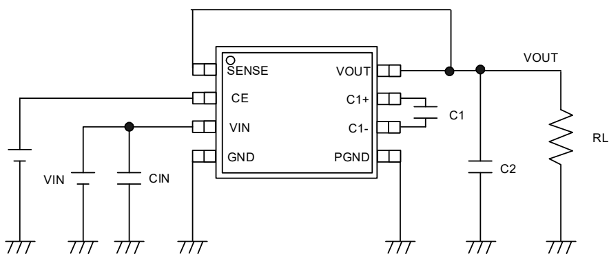
CIRCUIT③
