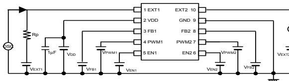
Circuit ⑦
