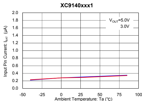
(6) Input Pin Current vs. Ambient Temperature
