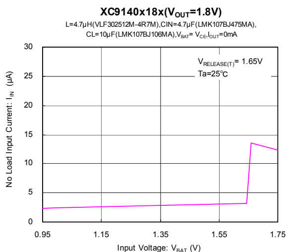
(21) No Load Input Current vs. Input Voltage
