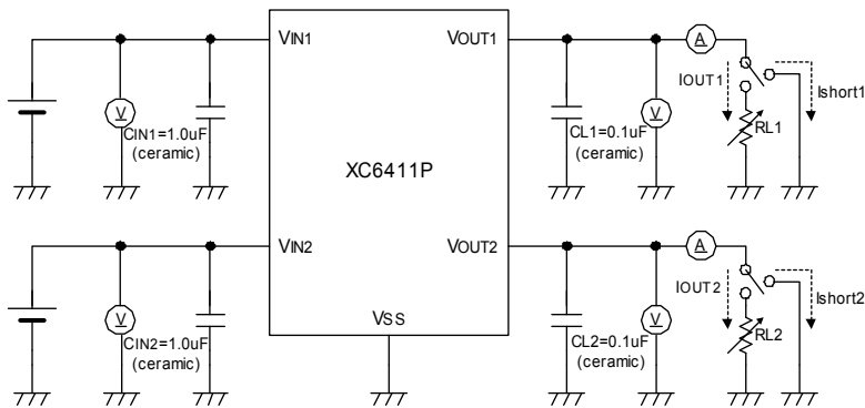
Circuit ①
