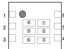
DFN1515-6A
