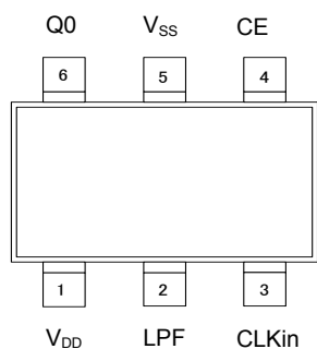
SOT-26W (TOP VIEW)
