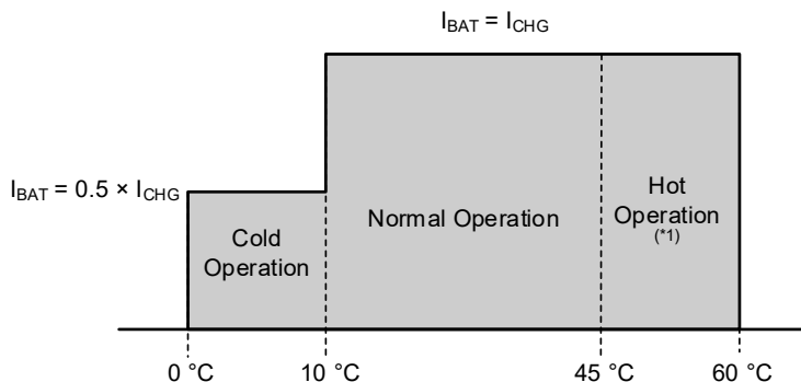
Constant-Current Charge vs. Thermistor Temperature
