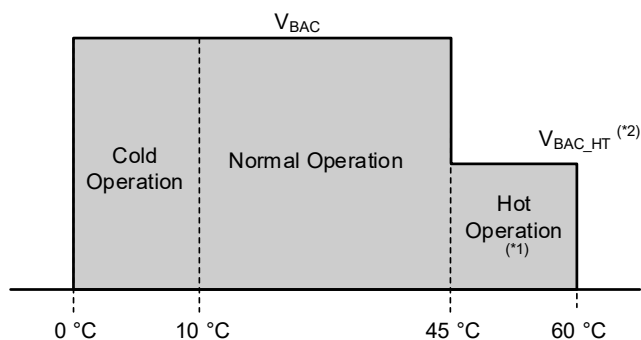
Constant-Voltage Charge vs. Thermistor Temperature
