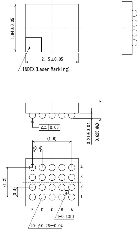
WLP-20-01 Recommended Pattern Layout (Reference)
