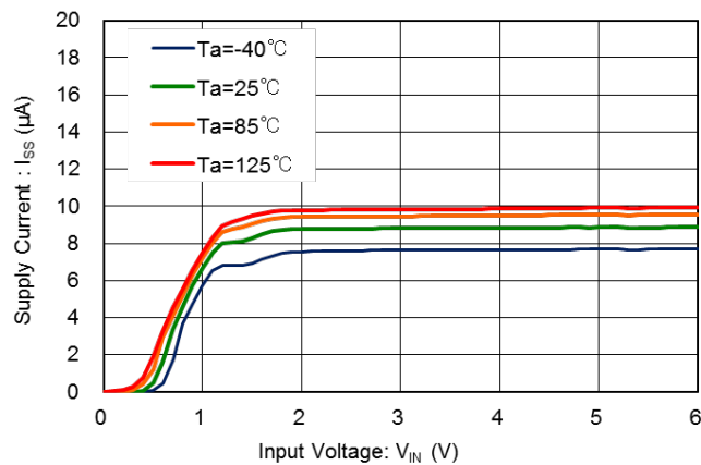
XD6130 ( V_{DF(T)}=5.0V )
