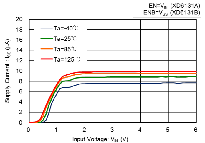
XD6131 ( V_{DF(T)}=5.0V )
