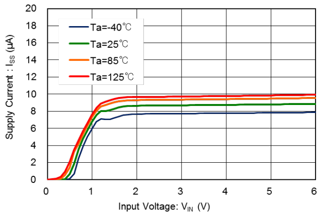
XD6130 ( V_{DF(T)}=1.6V )
