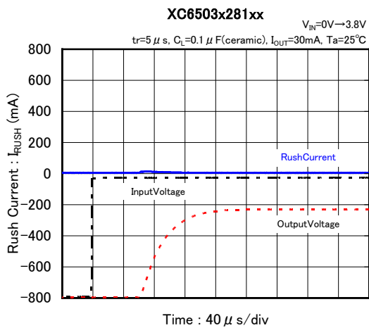
(7) Rush Current
