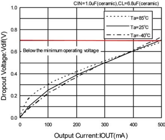
XC6210 (VOUT:0.8V)
