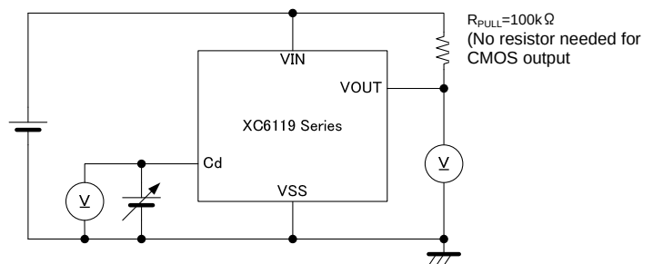
Circuit 8
