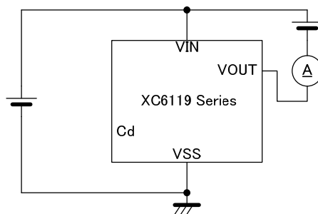
Circuit 6
