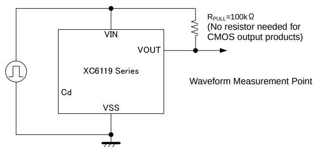
Circuit 8
