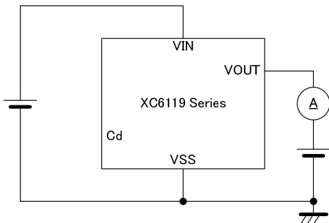
Circuit 5
