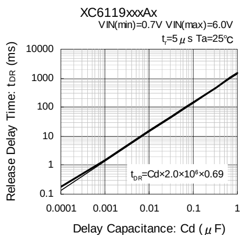
(8) Release Delay Time vs. Delay Capacitance
