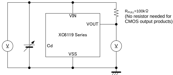
Circuit 3
