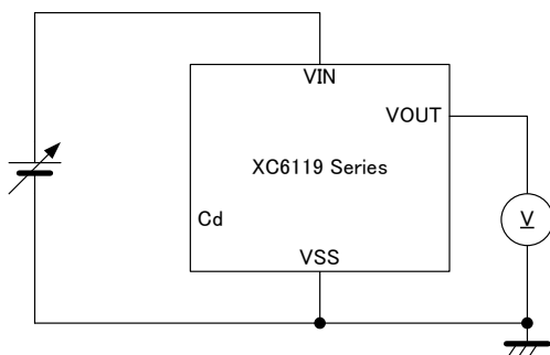
Circuit 7
