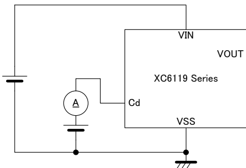
Circuit 7
