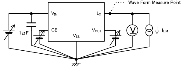
< Circuit No.6 >
