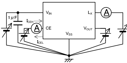
< Circuit No.5 >
