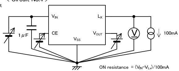
< Circuit No.4 >
