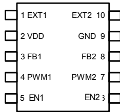
MSOP-10 (TOP VIEW)
