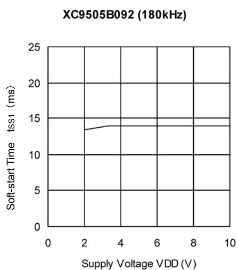
(20) Soft-start Time vs. Supply Voltage
