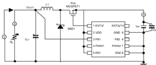
Circuit ③
