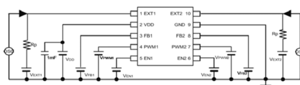
Circuit ⑥
