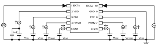
Circuit ③
