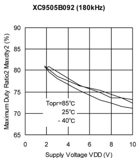
(19) MAX. Duty Ratio 2 vs. Supply Voltage
