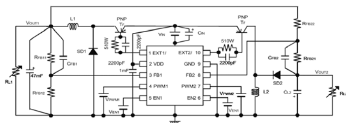
Circuit ②
