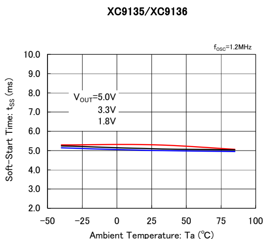
(12) Soft-Start Time vs. Ambient Temperature
