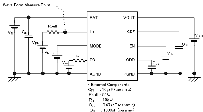
< Circuit No.6>
