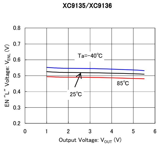
(16) EN "L" Voltage vs. Output Voltage
