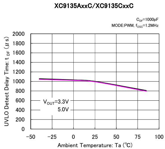
(25) UVLO Detect Delay Time vs. Ambient Temperature
