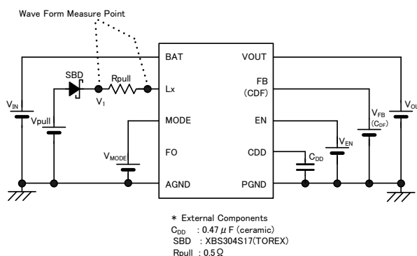
<Circuit No.9 >
