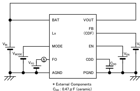
<Circuit No.7 >
