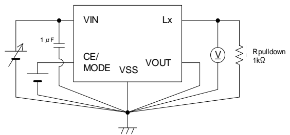
Circuit②
