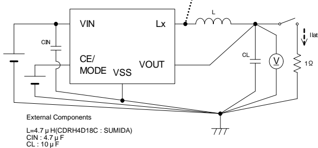
Circuit⑨
