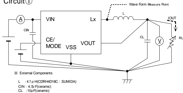
Circuit①
