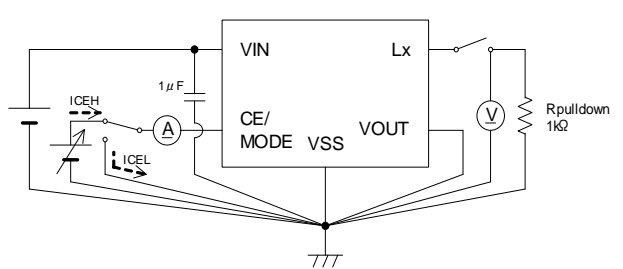
Circuit⑧
