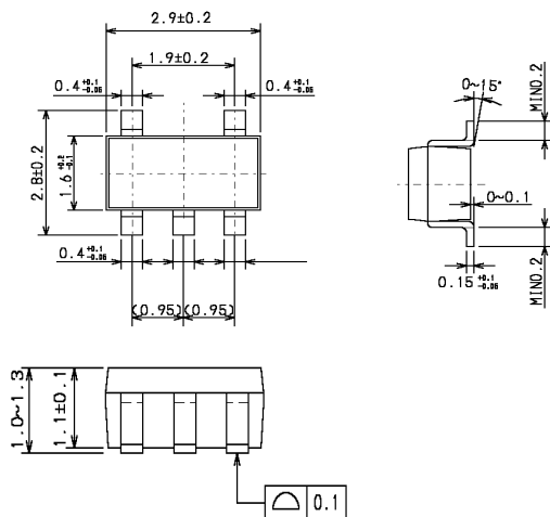
SOT-25 (SOT-23-5)
