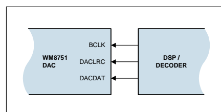
Figure 13 Slave Mode
