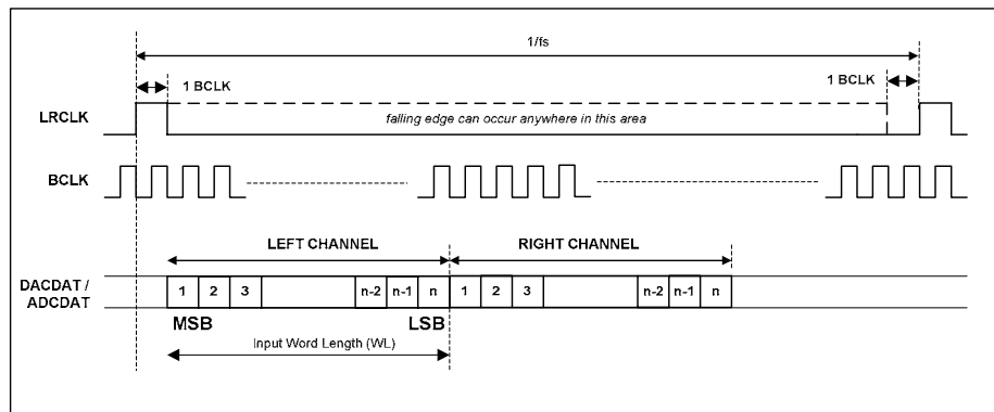
Figure 19 DSP/PCM Mode Audio Interface (mode A, LRP=0, Slave)
