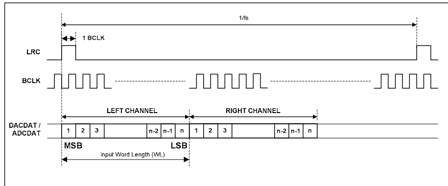
Figure 18 DSP/PCM Mode Audio Interface (mode B, LRP=1, Master)
