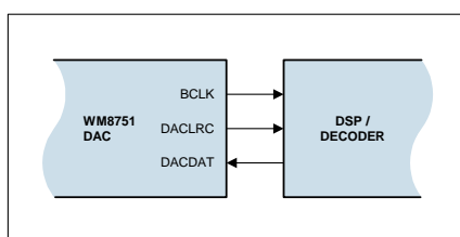
Figure 12 Master Mode
