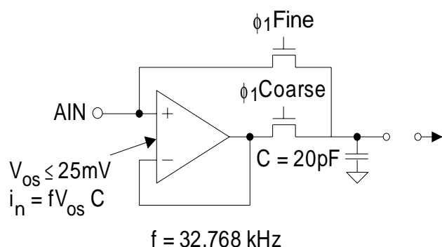
Figure 1. Input models for AIN+ and AIN- pins.
