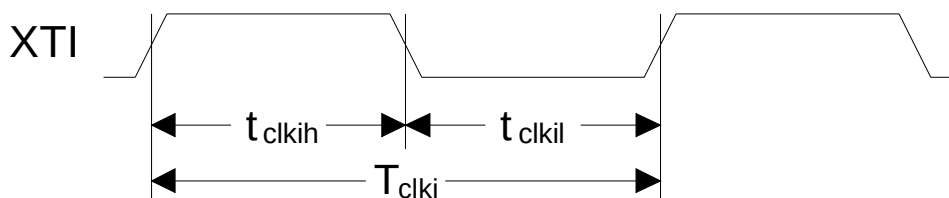
Figure 2. XTI Timing
