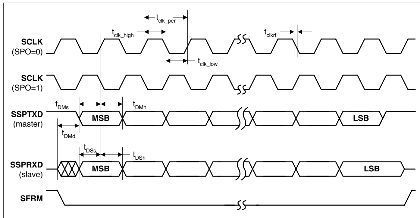
Figure 32. SPI Format with SPH=1 Timing Measurement
