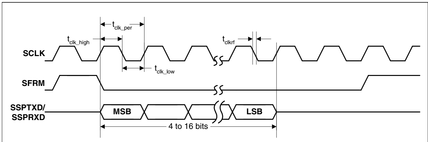
Figure 30. TI Single Transfer Timing Measurement
