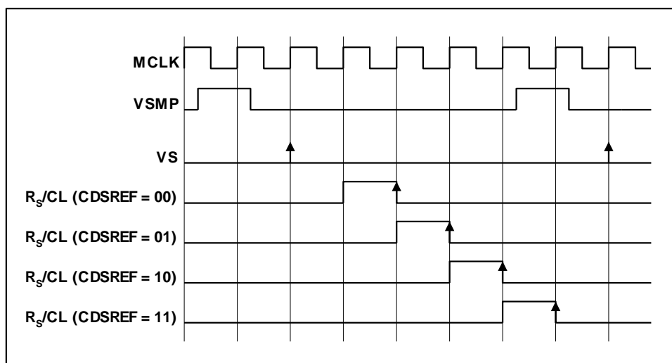
Figure 9 Reset Sample and Clamp Timing
