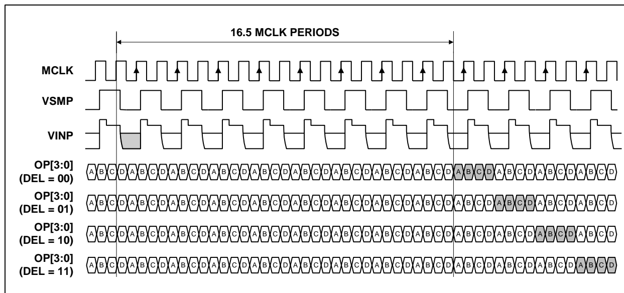
Figure 20 Mode 3 Operation
