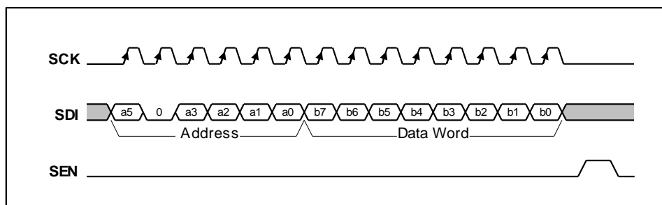
Figure 15 Serial Interface Register Write
