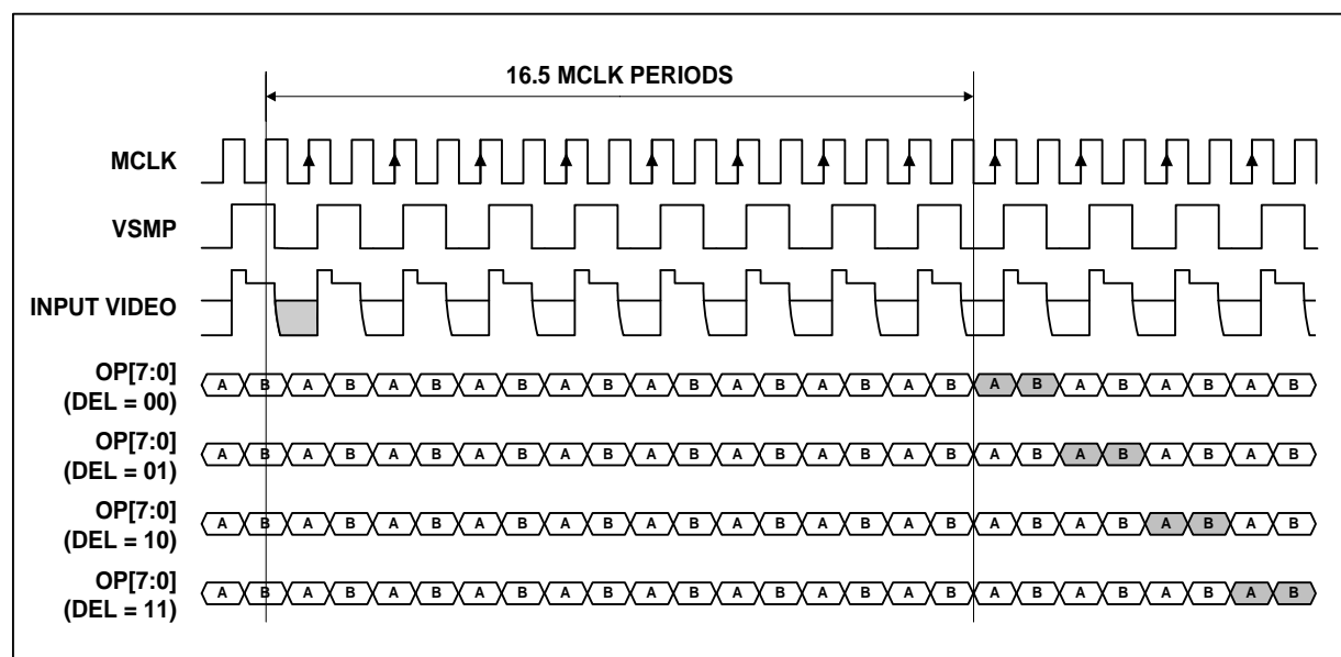
Figure 24 Mode 4 Operation
