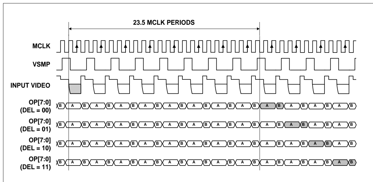
Figure 23 Mode 3 Operation
