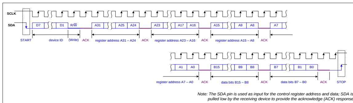
Figure 79 Control Interface 2-wire (I2C) Register Write (16-bit Data Words)
