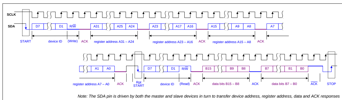
Figure 80 Control Interface 2-wire (I2C) Register Read (16-bit Data Words)
