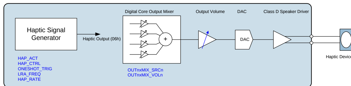
Figure 35 Digital Core Haptic Signal Generator
