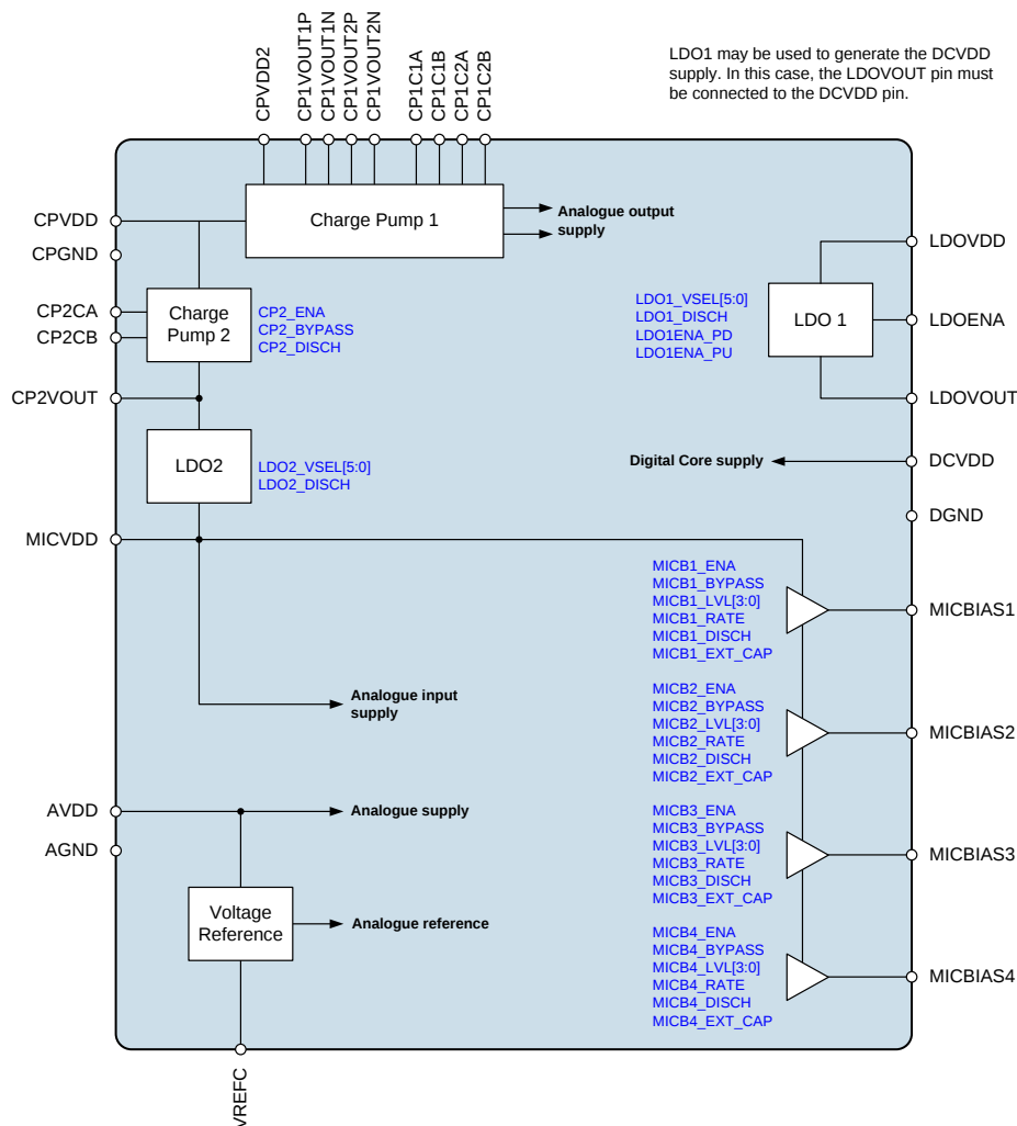
Figure 86 Charge Pumps and Regulators
