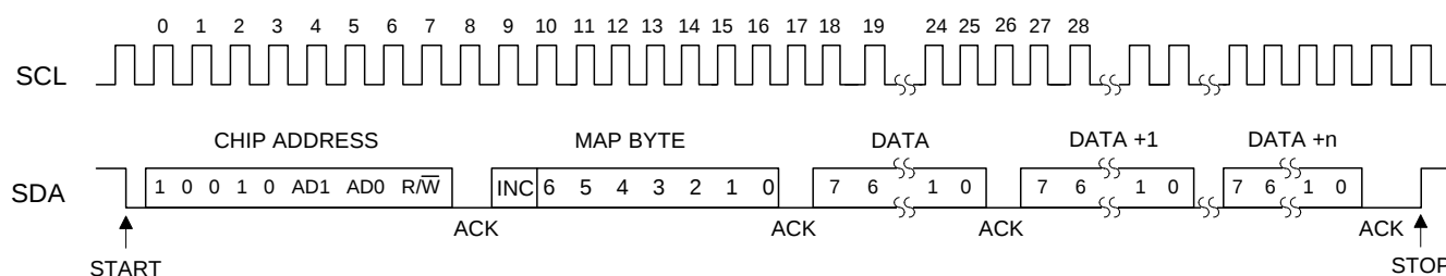
Figure 19. Control Port Timing, I²C Mode
