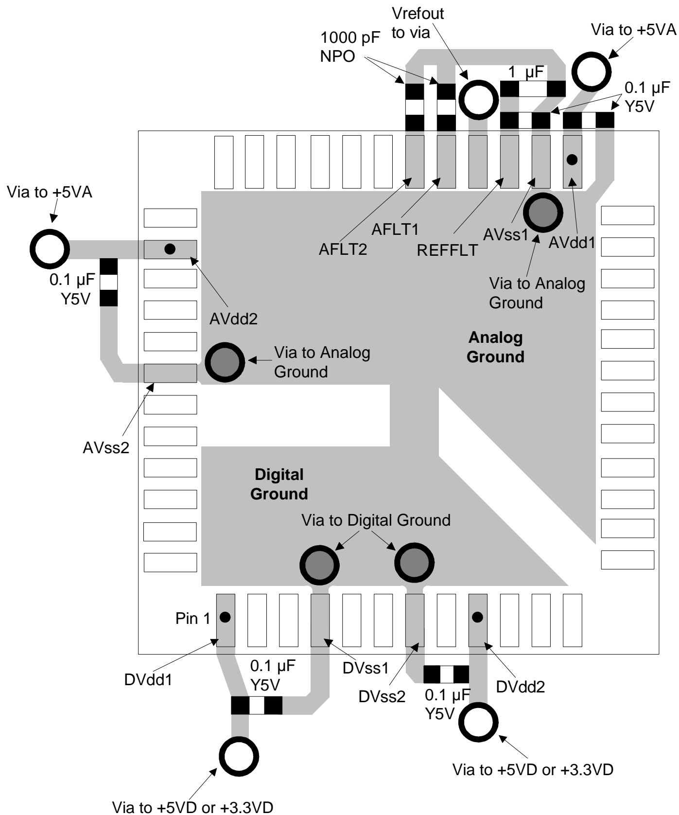
Figure 8-1. Conceptual Layout for the CS4299
