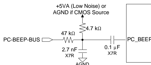
Figure 6-5. PC_BEEP Input
