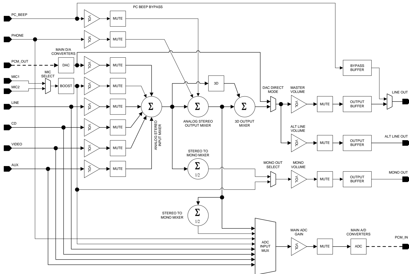
Figure 2-2. Mixer Diagram
