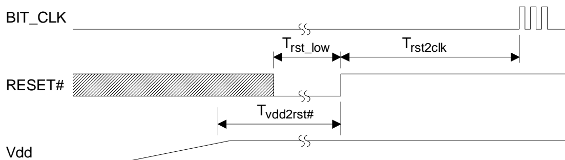
Figure 1-1. Power Up Timing
