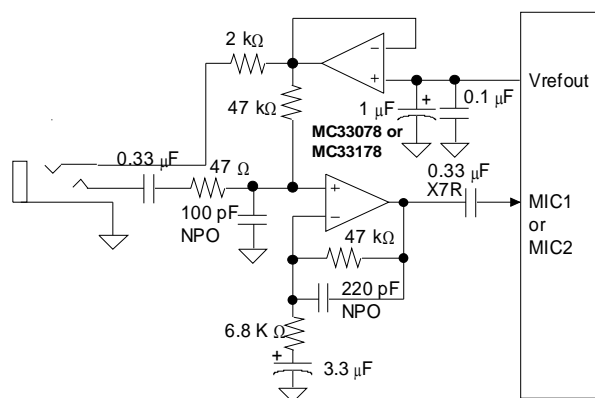
Figure 6-3. Microphone Input
