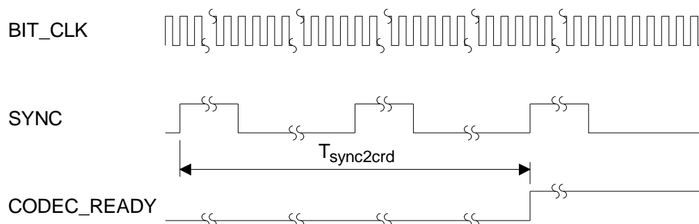
Figure 1-2. Codec Ready from Startup or Fault Condition
