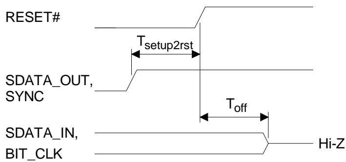
Figure 1-6. Test Mode
