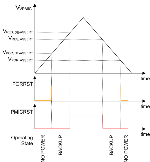
Figure 31 VPMIC Monitoring
