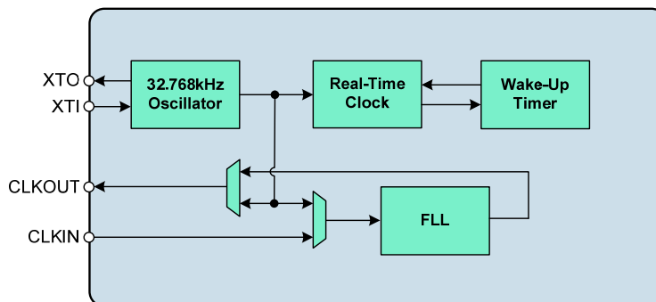
Figure 16 Clocking Configuration
