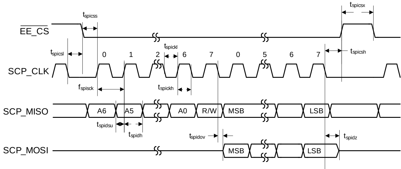
Figure 4. Serial Control Port - SPI Master Mode Timing
