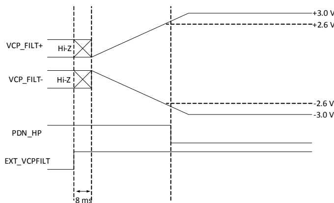
Figure 4-7. External VCP_FILT Power-Up Sequence
