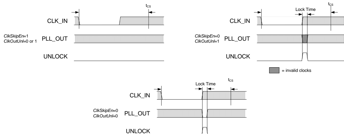
Figure 8. CLK_IN removed for < t_{cs}
