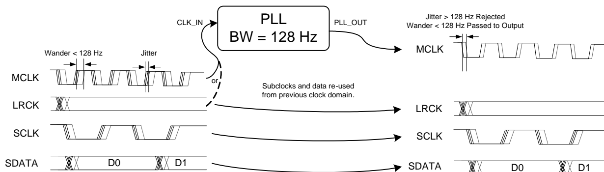
Figure 10. High bandwidth with CLK_IN domain re-use
